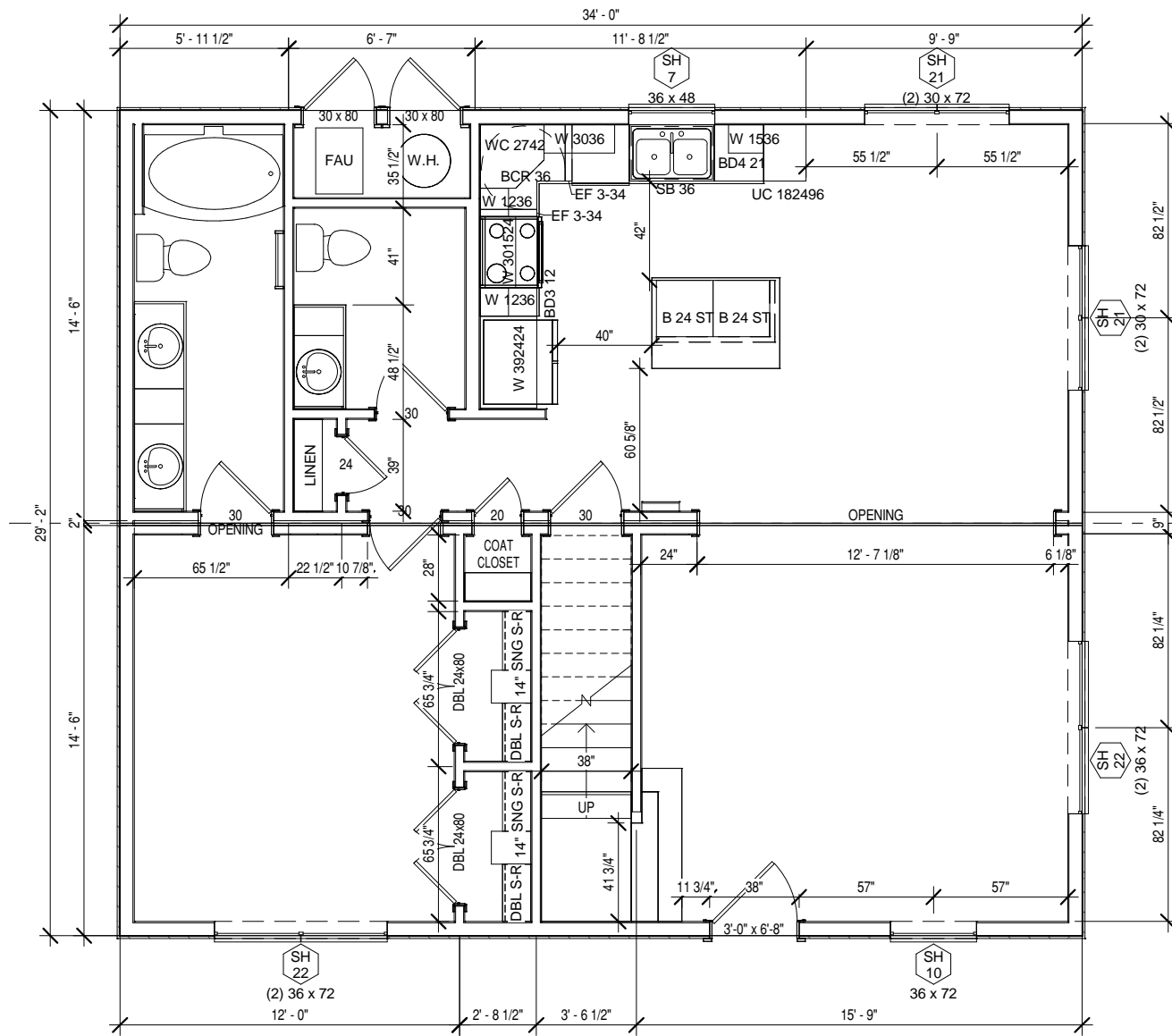
① L1-DECK 1/4" = 1'-0"
