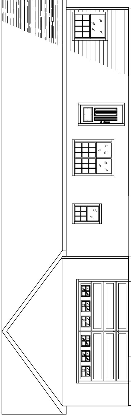
FRONT ELEVATION
